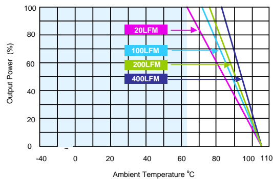
MTQZ50-72S05,MTQZ50-110S05 Derating Curve without Heatsink
