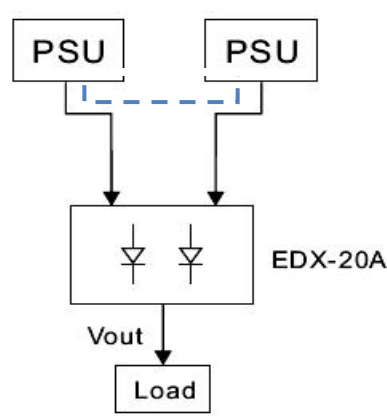
3.3 1+N 冗余接线图 1+N Redundancy Connection Diagram:
