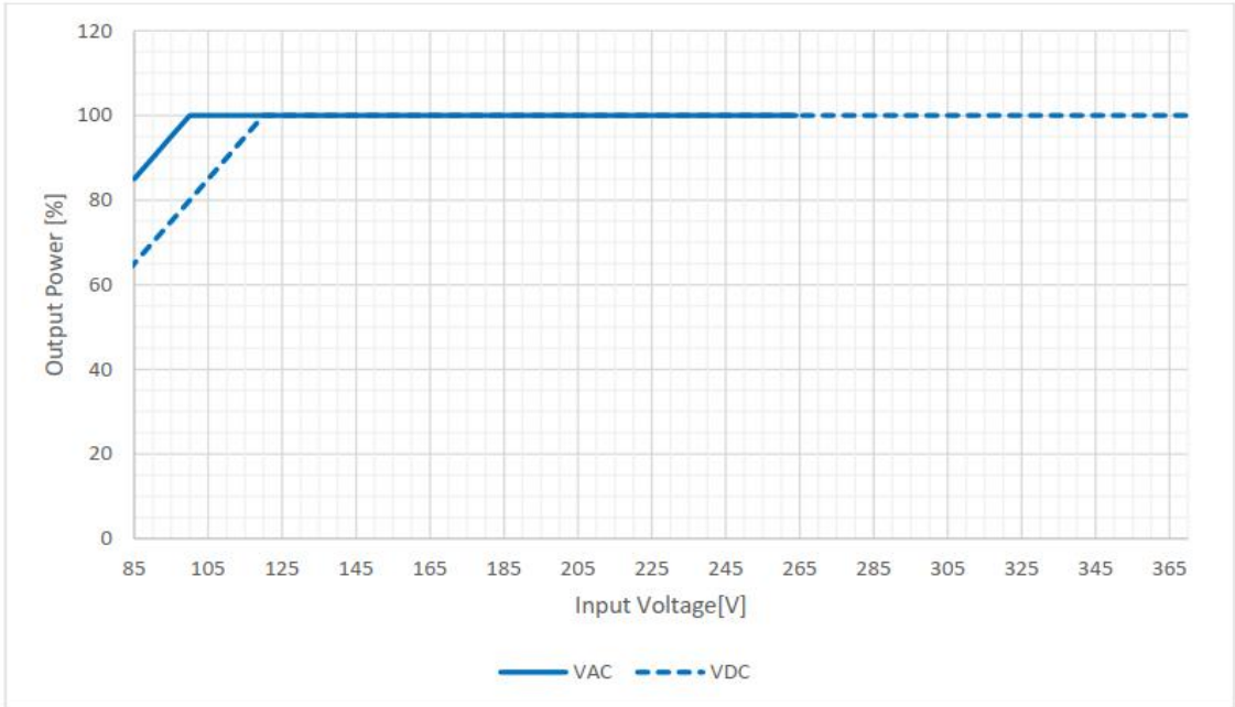
图1：输入电压下输出功率降额曲线 Fig1: Output Power Derating curve depending on Input Voltage
