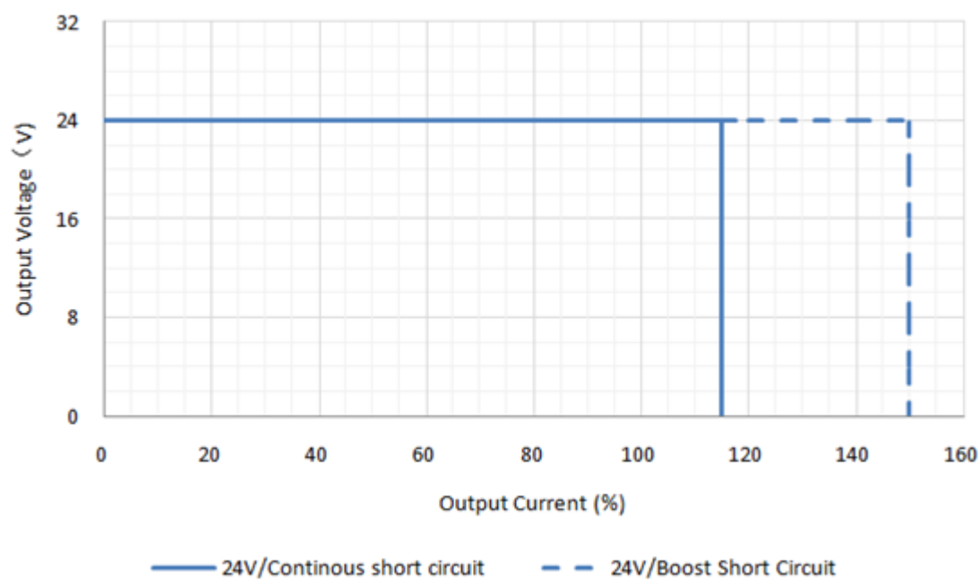
图1：正常输出电压下，正常和峰值工作时的限流曲线 Fig 1:Current limiting curve in normal and Boost operation depending on the nominal output voltage
